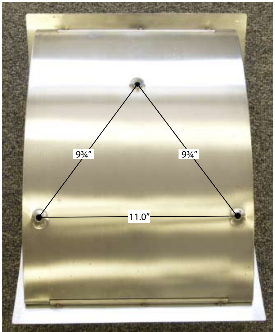
Capella Rear View, Mounting Holes
